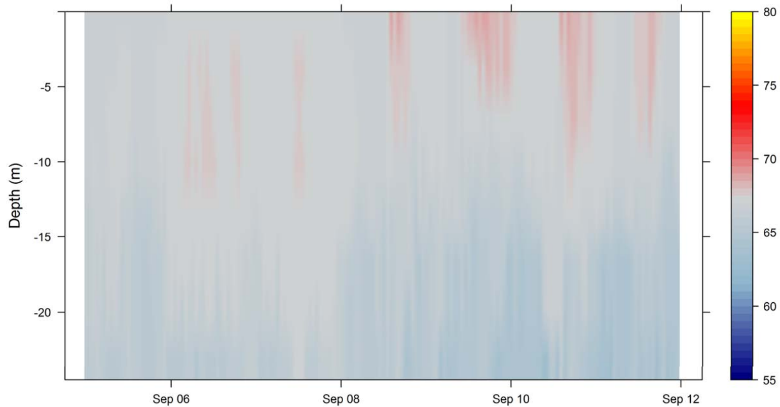
Figure 4 Water Temperatures in the Forebay for Week 36
