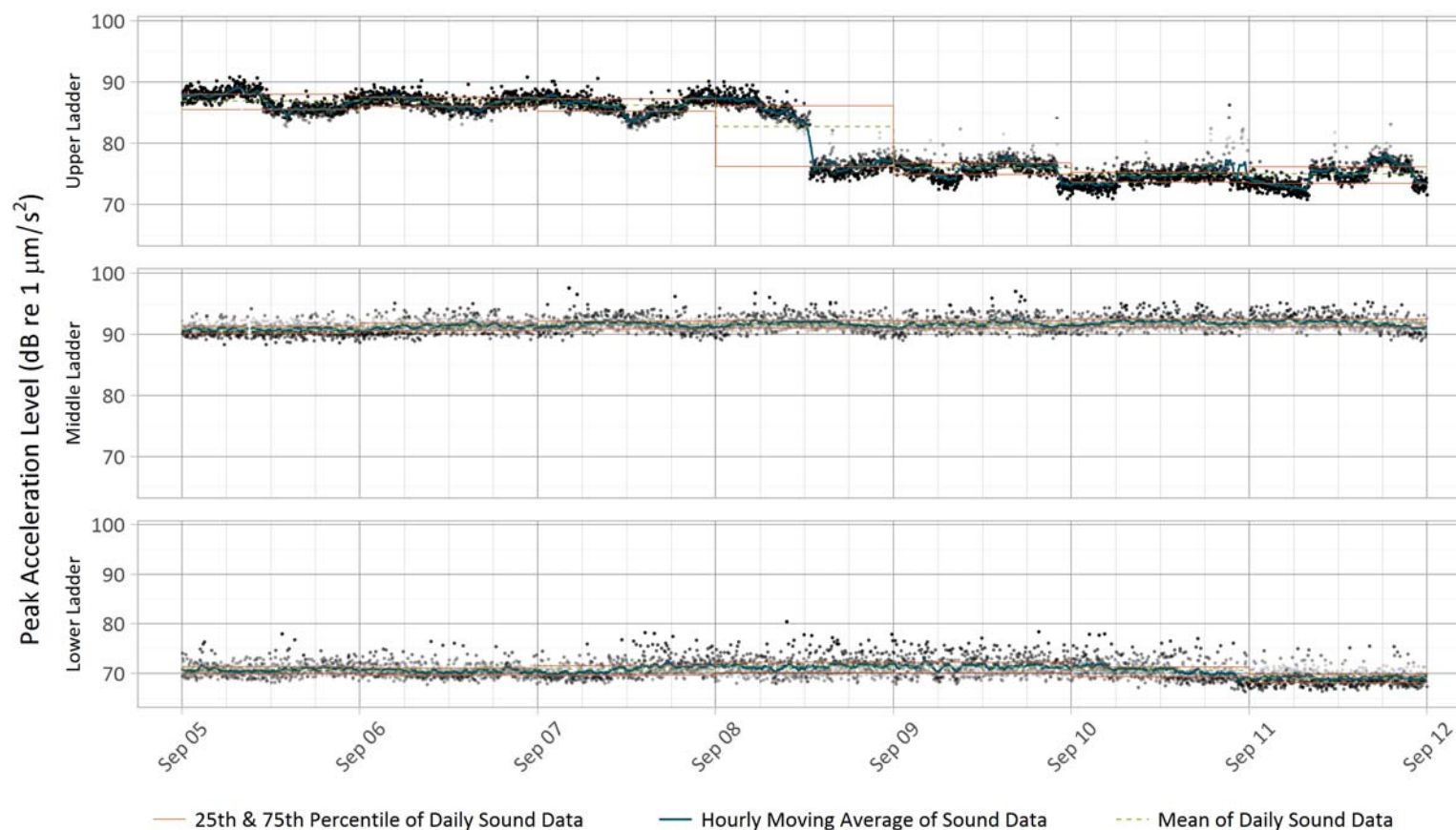
Figure 1 Peak Acceleration Levels Measured by Triaxial Accelerometers for Week 36
