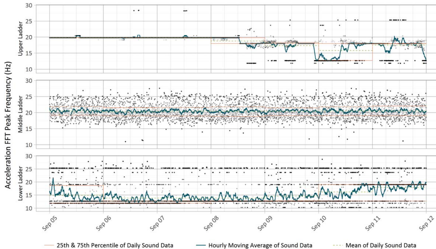
Figure 2 Acceleration Peak Frequencies Measured by Triaxial Accelerometers for Week 36
